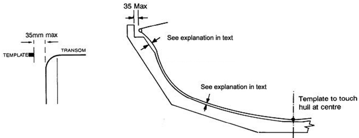
Hull Profile
